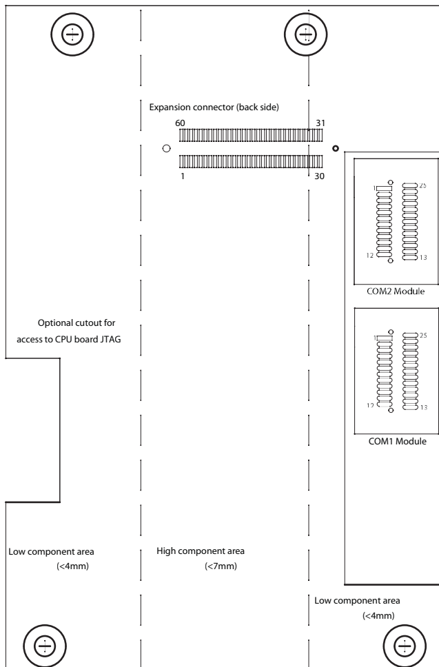
View looking into back of unit
